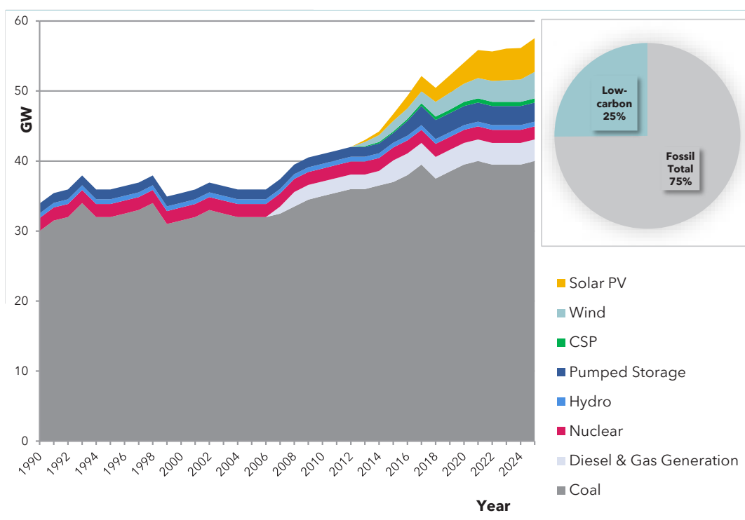
Figure 8. South Africa Historic Generation Capacity by Technology, GW vii
