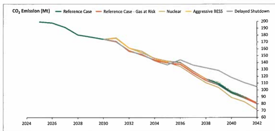
Figure 19: CO 2 Emissions Trajectory (Mt).
