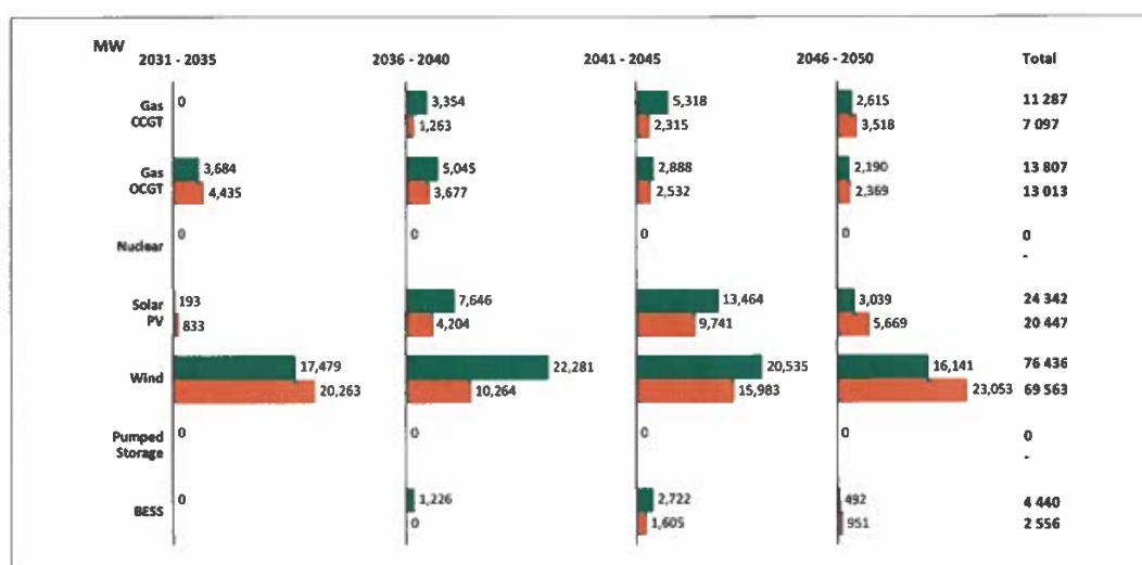
Figure 17: Reference Case and Delayed Coal Shutdown.
